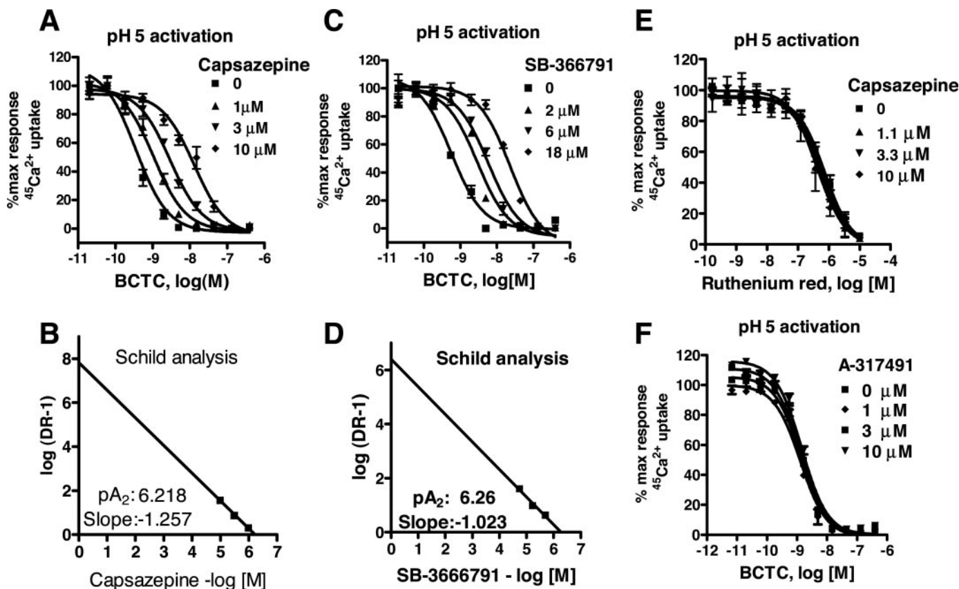
Fig. 3. A, concentration-response curves for BCTC inhibition of proton-induced ^{45}\text{Ca}^{2+} uptake into CHO cells expressing rat TRPV1 in the absence or presence of 1, 3, or 10 \mu\text{M} capsazepine. B, Schild analysis of competitive interaction between BCTC and 1.11 to 10 \mu\text{M} capsazepine. C, concentration response curves for BCTC inhibition of proton-induced ^{45}\text{Ca}^{2+} uptake into CHO cells expressing rat TRPV1 in the absence or presence of 3, 10, or 30 \mu\text{M} SB-366791. D, Schild analysis of competitive interaction between BCTC and 2 to 18 \mu\text{M} SB-366791.
