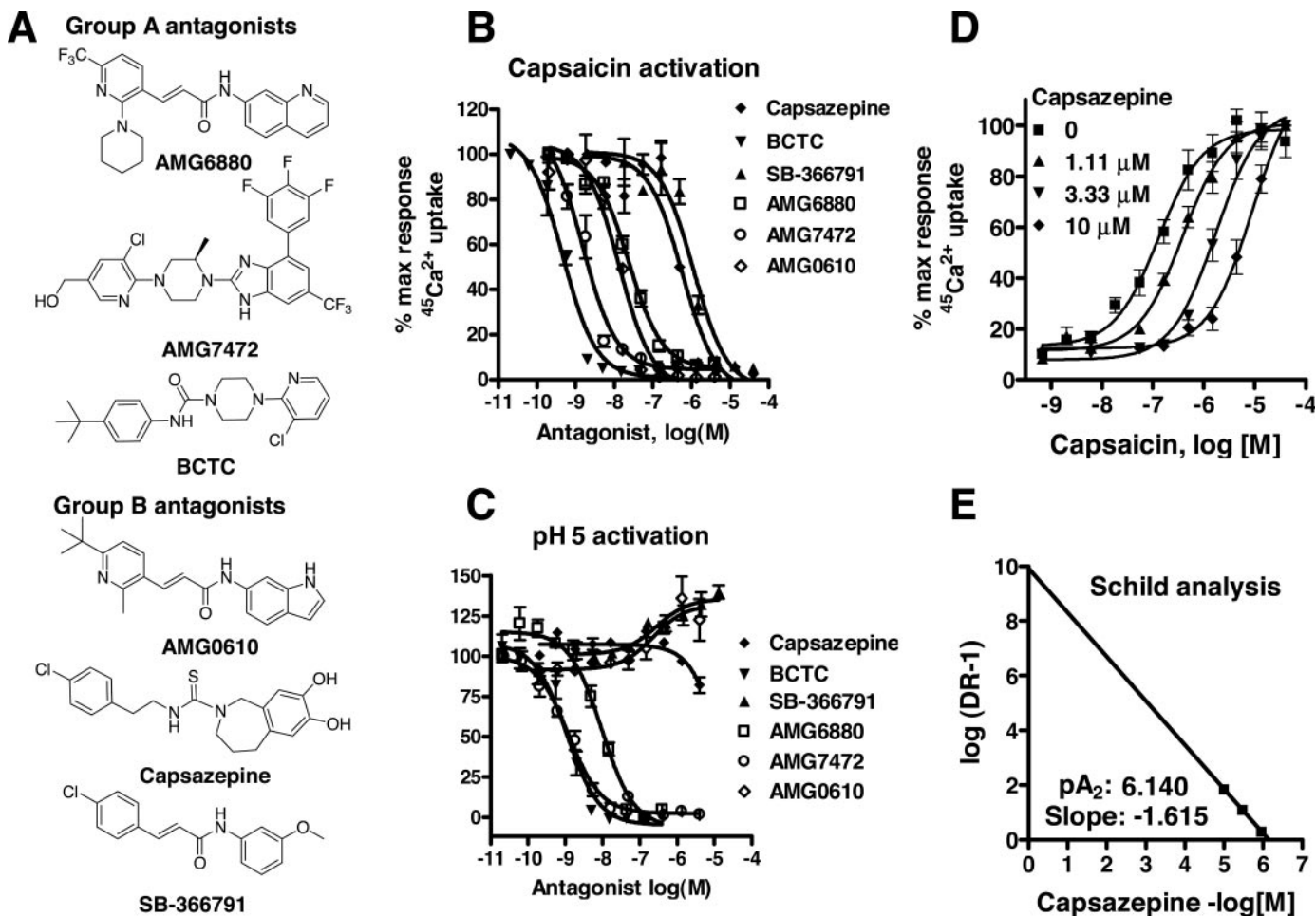
Fig. 1. Structures of antagonists used in the study are shown in A. Comparison of antagonists for inhibition of capsaicin (0.5 \mu\text{M} ) (B) and proton (pH 5) (C) induced activation of rat TRPV1. CHO cells stably expressing rat TRPV1 were used in agonist-induced ^{45}\text{Ca}^{2+} uptake assay as described under Materials and Methods . Cells were incubated for 2 min with increasing concentrations of antagonists as indicated, followed by the addition of agonists for additional 2 min. Each point in the graph is an average \pm S.D. of an experiment conducted in triplicate. Please note potentiation of pH 5-induced ^{45}\text{Ca}^{2+} uptake above 100% by SB-366791 at high concentrations (>10 \mu\text{M} ) in C. \text{IC}_{50} values for capsaicin and pH 5 activation are shown in Table 2. D, concentration-response curves for capsaicin-induced ^{45}\text{Ca}^{2+} uptake into CHO cells expressing rat TRPV1 in the absence or presence of 1.11, 3.33, or 10 \mu\text{M} capsazepine. E, Schild analysis of the antagonism produced by 1.11 to 10 \mu\text{M} capsazepine.
