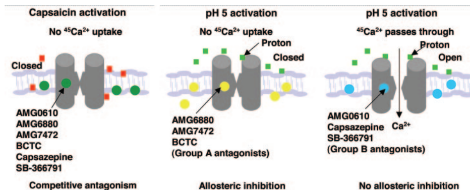
Fig. 5. Models of agonist and antagonist interaction with capsaicin-binding pocket of rat TRPV1. Left, capsaicin binds the intramembrane vanilloid-binding pocket constituted by the TM3/4 region. Antagonists such as AMG0610, AMG6880, AMG7472, BCTC, capsazepine, and SB-366791 compete with capsaicin for the same binding pocket. Middle, critical residues for proton activation are located at the prepore loop. Antagonists such as AMG6880, AMG7472, and BCTC (group A) bind at the capsaicin-binding pocket and stabilize or lock the channel conformation in the closed or nonconducting state even when protons are present at pH 5 (it is not known whether group A antagonist binding prevents protonation of TRPV1). Right, AMG0610, capsazepine, and SB-366791 (group B) bind the same pocket as group A antagonists but do not stabilize or lock channel conformation in the closed or nonconducting state. Proton activation (pH 5-induced conformational changes) occurs while the group B antagonists are bound to the channel and 45 Ca 2+ passes through. Capsaicin and protons are shown in red and green squares, respectively. All antagonists (●) are shown in green (left), group A antagonists are shown in yellow (middle), and group B antagonists are shown in blue (right).
