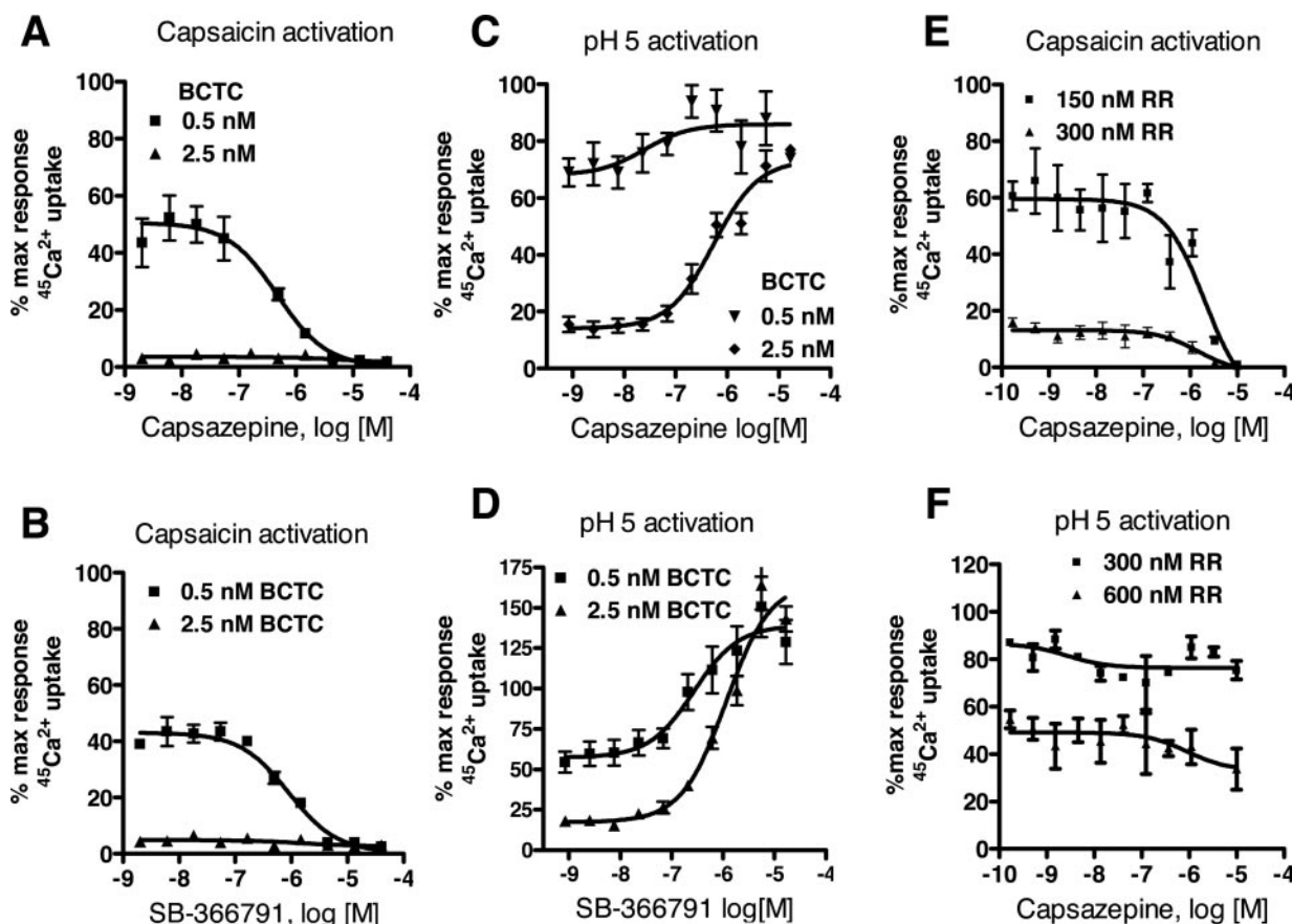
Fig. 2. Concentration-dependent inhibition of capsaicin activation by mixtures of capsazepine and BCTC (A) or SB-366791 and BCTC (B) or capsazepine and ruthenium red (RR) (E). Note the remaining capsaicin-induced ^{45}\text{Ca}^{2+} uptake in the presence of BCTC (0.5 nM) or 150 nM RR inhibition was inhibited in a concentration-dependent manner by capsazepine and SB-366791, indicating additive antagonism. Capsazepine (C) and SB-366791 (D) compete with BCTC and prevent BCTC inhibition of rat TRPV1 activation by protons. Note that BCTC inhibition of proton-induced ^{45}\text{Ca}^{2+} uptake is prevented in a concentration-dependent manner by both capsazepine and SB-366791 (C and D); however, capsazepine did not affect RR inhibition of proton-induced ^{45}\text{Ca}^{2+} uptake (F). \text{IC}_{50} values for capsazepine and SB-366791 blockade of 2.5 nM BCTC inhibition of rat TRPV1 activation by protons are 0.55 \pm 0.07 and 1.15 \pm 0.09 \mu\text{M} , respectively. At higher concentrations ( >0.3 \mu\text{M} ), SB-366791 potentiation is represented by an increase of ^{45}\text{Ca}^{2+} uptake above 100% (D).
